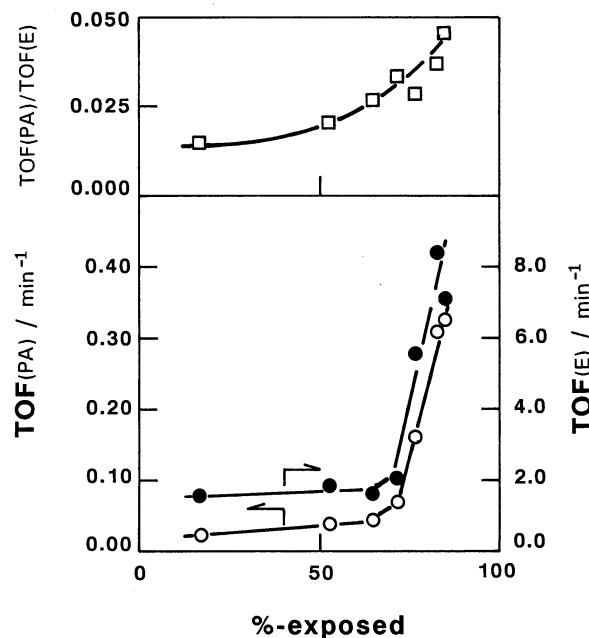
Fig. 2. Effects of Pd dispersion on the catalytic behavior of Pd/SiO 2 for ethylene hydroformylation (at 373 K). ○, TOF(PA); ●, TOF(E); □, TOF(PA)/TOF(E).
